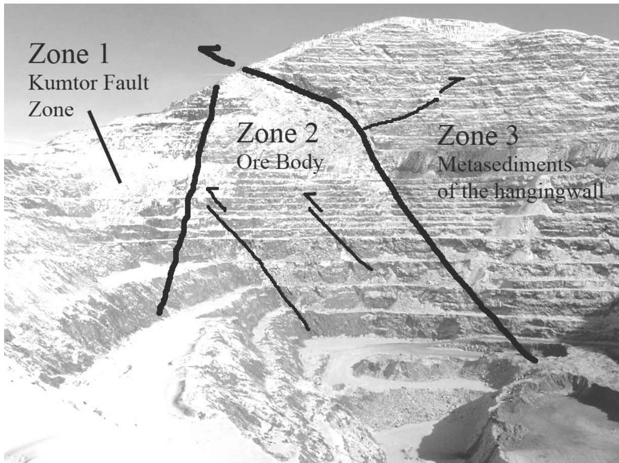
Figure 2 Photograph showing the main tectonic zones and the zone bounding faults in the North wall of the Kumtor central pit
