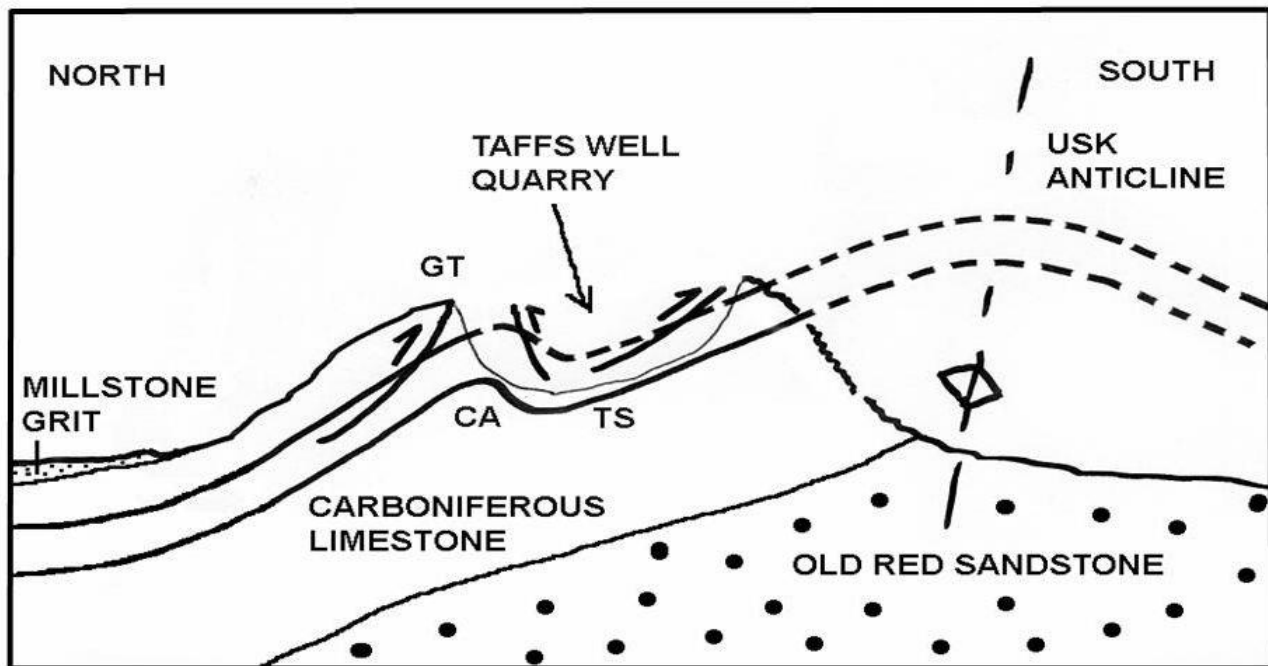
Figure 7 The geology of the Taffs Well area showing its structural position within the regional cross section. CA – Castell Coch Anticline, TS – Tongwynlais Syncline and GT – Pen-y-Garn Thrust. (NB - section is not to scale)
