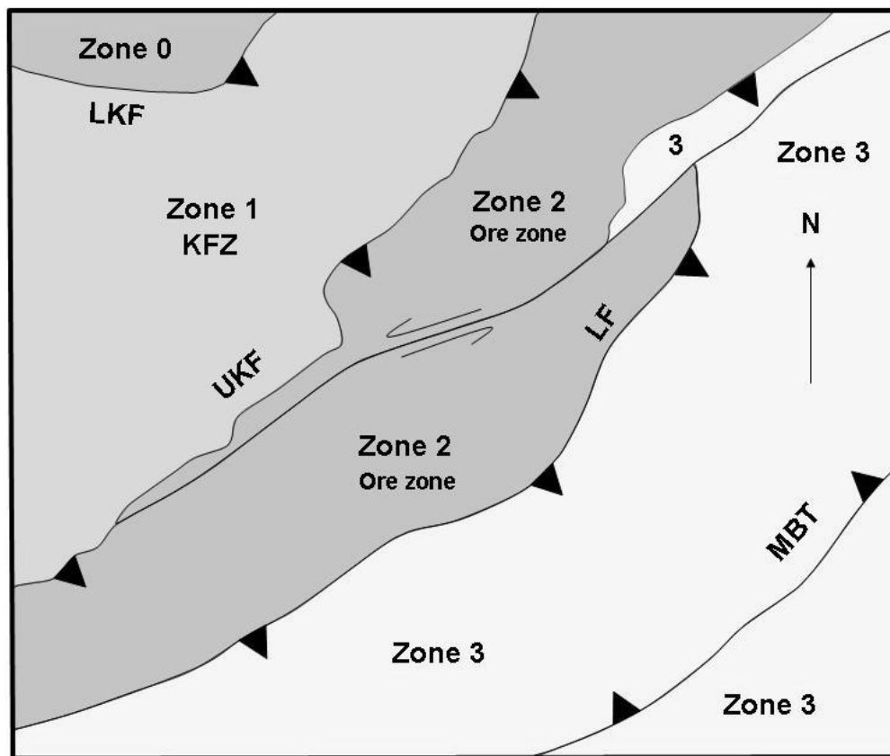
Figure 4 Sketch geological map of the Kumtor central pit area showing main tectonic zones and faults. LKF – Lower Kumtor Fault, UKF Upper Kumtor Fault, LF – Lysi Fault and MBT – Main Back Thrust. KFZ – Kumtor Fault Zone
